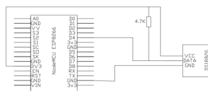
Gambar 4. Rangkaian Sistem Monitoring Suhu
