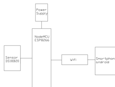
Gambar 2. Blok Diagram Sistem Monitoring Suhu
