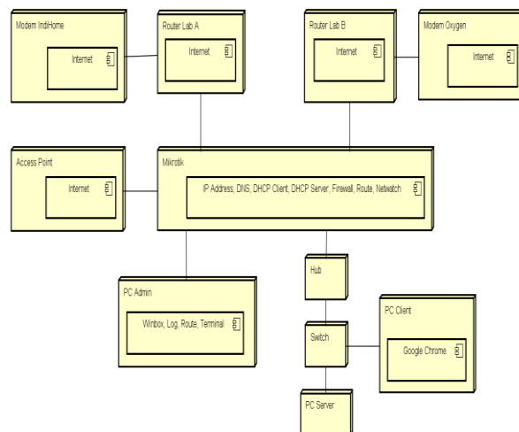
Gambar 6. Deployment diagram Usulan
