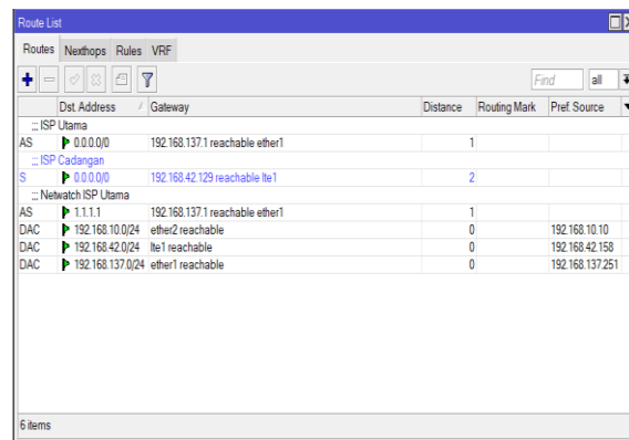
Gambar 15. Tampilan Route
