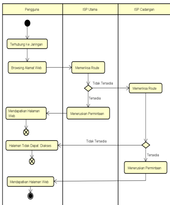
Gambar 5. Activity diagram Usulan
