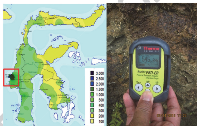
Fig. 1. Study site, Mamuju District, West Sulawesi Province (red rectangle) of Sulawesi Island with its radioactivity mapping in nSv/h (left) 39) and result of environmental radioactivity measurement with a detector in area showing 545 \mu R/h of dose rate (right).
