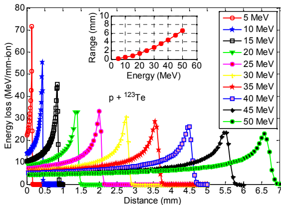
Fig. 7 SRIM-calculated energy loss and range of various energetic proton beams in ^{123}\text{Te} target.
