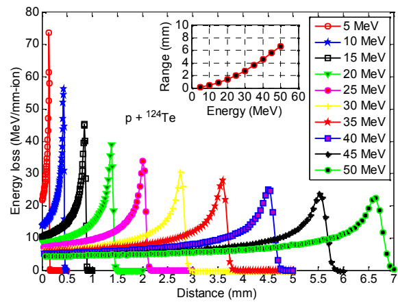
Fig. 8 SRIM-calculated energy loss and range of various energetic proton beams in ^{124}\text{Te} target.
