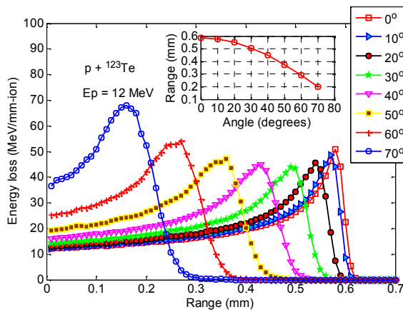
Fig. 9SRIM-calculated energy loss and range of a 12-MeV proton beam in ^{123}\text{Te} target at varied incidence angles.
