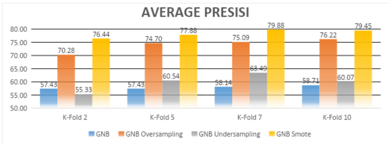
Gambar 6. Hasil rata-rata presisi Gaussian Naïve Bayes
