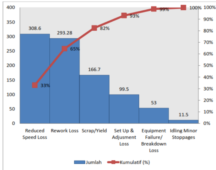
Gambar 3. Diagram pareto
