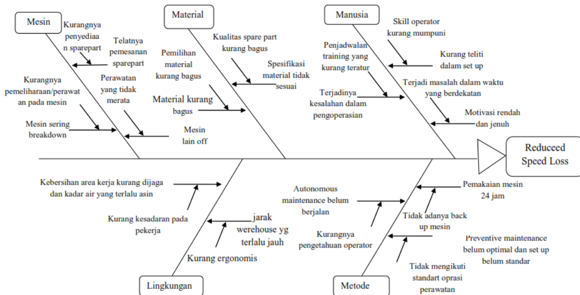
Gambar 4. Diagram fishbone
