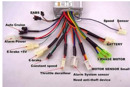
Gambar 6 Controller Universal
