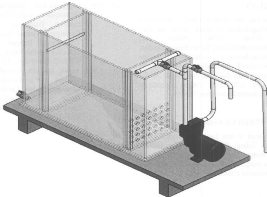
Gambar 1.3 Subsurface Flow Constructed Wetland Tampak Keseluruhan
