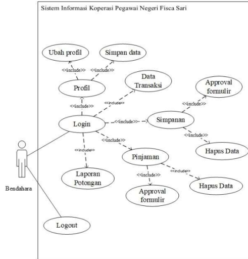
Gambar 4. Use case diagram bendahara
