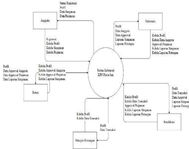
Gambar 2. Data Flow Diagram (Context Diagram)
