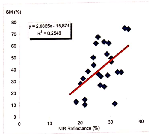
Fig. 2. Response of NIR Reflectance (R2) vs Soil Moisture
