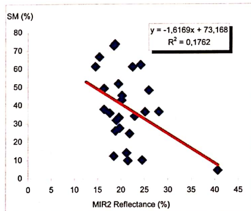
Fig. 6. Response of MIR 2 Reflectance (R6) vs Soil Moisture
