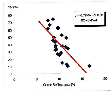
Fig. 4. Response of Green Reflectance (R4) vs Soil Moisture
