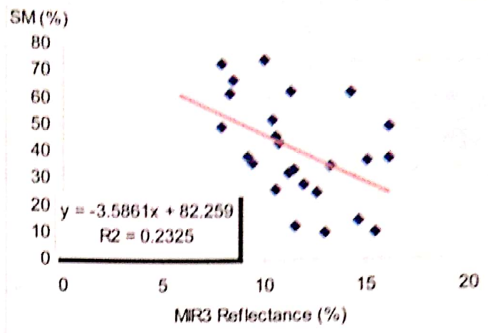
Fig. 7. Response of MIR 3 Reflectance (R7) vs Soil Moisture
