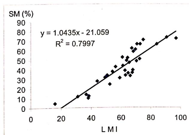
Fig. 8. Scatter plot and Trend between Soil Moisture and Land Moisture Index
