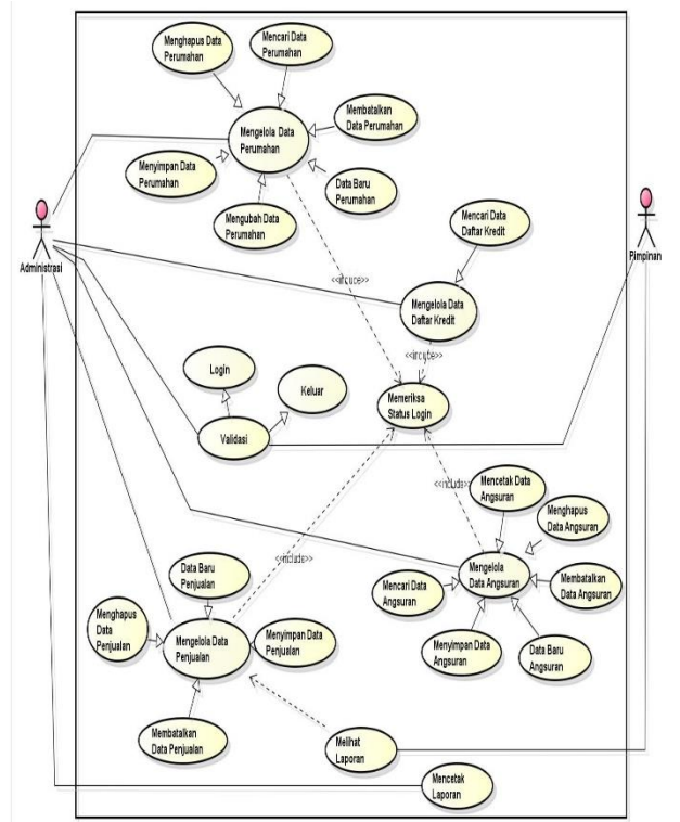
Gambar 1. Desain Use Case Diagram
