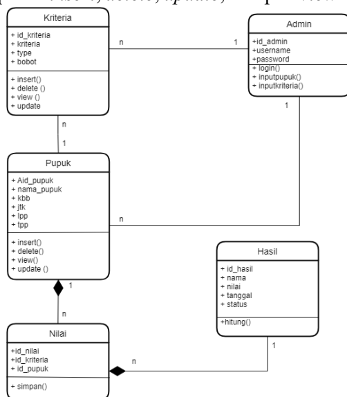
Gambar 10. Class Diagram
