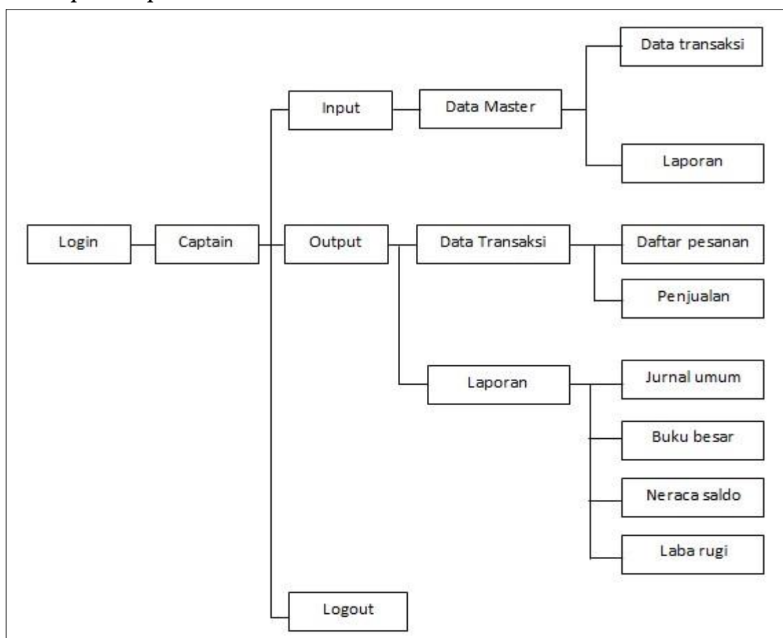
Gambar 5. Struktur menu captain
