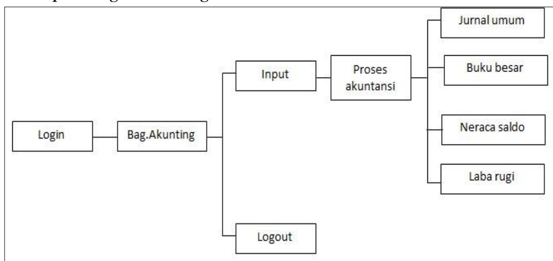
Gambar 6. Srtuktur menu bag.akunting
