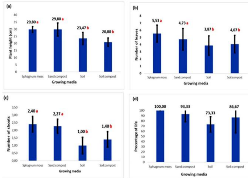
Fig.7. The effect of the growing media on plant height (a), number of leaves (b), number of shoots (c) and percentage of plant life (d) of H. borneense at the age of 3 months after planting (Trimanto et al. , 2019). Different lowercase letters (red colour) represent significant differences between different growing media applications.
