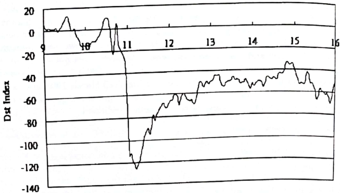
Figure 2-1: Variation of the geomagnetic index Dst during 9-15 March 1998
