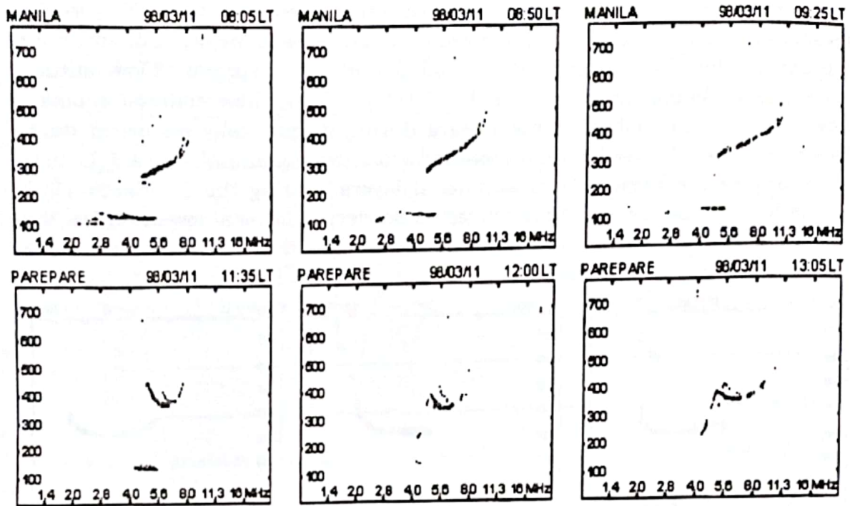
Figure 3-2: Selected ionograms recorded at Manila and Parepare on 11 March 1998
