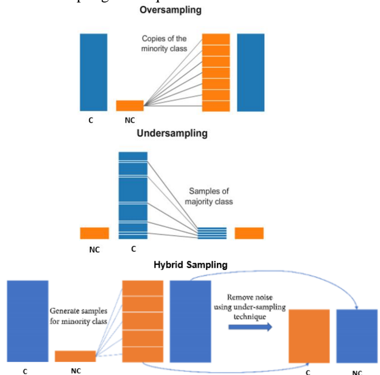
Fig. 2. The illustration of the resampling techniques
