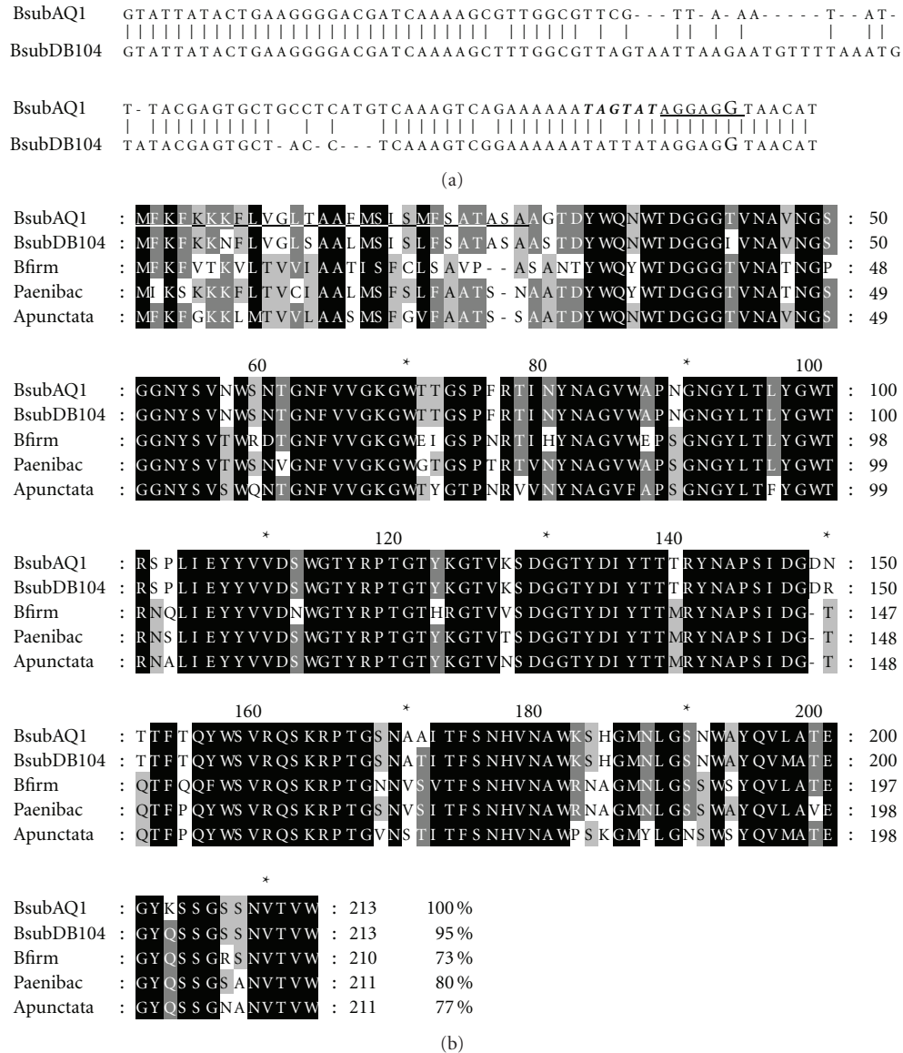
FIGURE 2: Alignment of AQ1 endoxylanase with other endoxylanases. (a) Comparison of putative promoter region endoxylanase gene of B. subtilis strain AQ1 and that of B. subtilis strain DB104. Underlined nucleotides correspond to the putative SD site, the large alphabet corresponds to the probable Transcription Start Site (TSS), the bold and italic nucleotides show the probable -10 sequence (b) Alignment of AQ1 endoxylanase’s deduced amino acid (this work) with BsubDB104 from Bacillus subtilis DB104 (this work) Bfirm from Bacillus firmus (AAQ83579); Paenibac from Paenibacillus sp. ([9]; DQ869568), and Apunctata from Aeromonas Punctata (D32065). In sequence of AQ1 endoxylanase underlined amino acids constitute the putative signal peptide.
