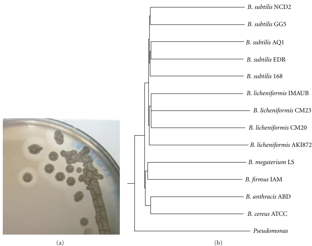
FIGURE 1: The morphology of newly isolated strain AQ1. Colony morphology on LB xylan agar medium (a) and its phylogenetic tree analyses (b).
