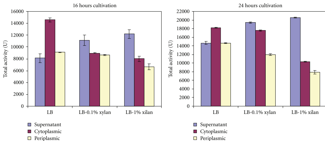
FIGURE 4: Recombinant AQ1 endoxylanase distribution in cellular compartment of E. coli after 16 and 24 hours of cultivation at 37°C of 25 mL medium culture at shaking erlenmeyer flask. The given values in all activity assays are the means of triplicates, and the error bars indicate the standard deviation of these triplicates of independent experiment.
