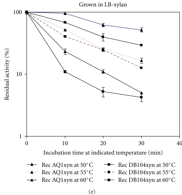
FIGURE 3: Recombinant E. coli with and without xylanase activity and the comparison of properties of AQ1 and DB104 recombinant xylanase. (a) Recombinant E. coli on LB xylan, recombinant E. coli harbouring empty pGEM-T-easy vector (1), recombinant E. coli with vector pGEM containing AQ1xyn without native promoter (2), recombinant E. coli with vector pGEM containing AQ1xyn with native promoter (3), and recombinant E. coli with vector pGEM containing DB104xyn with native promoter (4). (b) The molecular mass of recombinant AQ1 endoxylanase in E. coli . For this analysis, the expression of the xylanase gene in cytoplasmic fraction with T7 promoter was used. (c) Effect of temperature on recombinant AQ1 endoxylanase and DB104 endoxylanase grown in LB and LB-xylan medium (triangle was recombinant AQ1 xylanase, black one for that came from E. coli grown in LB-xylan, white one for that one grown in LB; square was DB104, black one for that one grown in LB-xylan, white one for that one grown in LB). For this temperature profile, enzymatic activity was measured in 50 mM sodium phosphate pH 7. (d) Effect of pH on recombinant AQ1 endoxylanase and DB104 endoxylanase from E. coli grown in LB and LB-xylan medium in different buffers. The reaction pHs were adjusted to 5–11 with the following buffers: 50 mM citrate buffer (pH 5,6), 50 mM phosphate buffer (pH 6–8), 50 mM Tris-HCl (pH 8–10), and 50 mM Tris-Glycine buffer (pH 10,11) (triangle was recombinant AQ1 xylanase, black one for that came from E. coli grown in LB-xylan, white one for that one grown in LB; square was recombinant DB104 xylanase, black one for that one grown in LB-xylan, white one for that one grown in LB). (e) Thermostability of recombinant AQ1 endoxylanase and DB104 endoxylanase. Thermostability was determined by preincubating enzyme extract at 50, 55, and 60°C for designated time periods and then assaying the activity in pH 7.0 of 50 mM sodium phosphate at 50°C for 5 min as described in Materials and Methods. The given values in all activity assays are the means of triplicates, and the error bars indicate the standard deviation of these triplicates of independent experiment.
