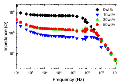
Fig. 2. Plot correlation frequency vs impedance
