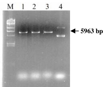
Figure 2. BamH I and Not I Digestion Against pYES2/CT. M. \lambda /Hind III Markers; Line 1. BamH I Digestion; Line 2. Not I Digestion; Line 3. BamH I and Not I Digestion. Line 4. Intact pYES2/CT. 0.8% Agarose gel (w/v), 75 Volt, EtBr 1 \mu g/mL
