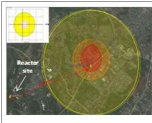
Figure 1. Fire area around Fuel Station[16]
