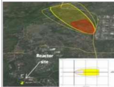
Figure 2. Explosion area around Fuel Station[16]
