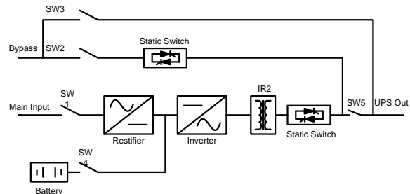
Gambar 1. Blok diagram sistem UPS AC
