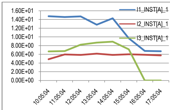
Gambar 6. Arus beban
