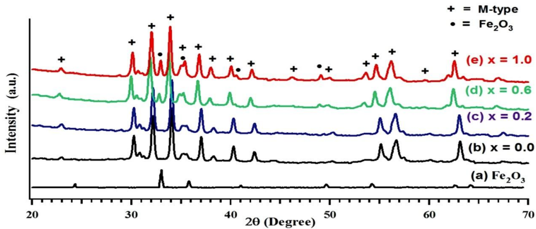
Figure 1. XRD pattern of \text{Fe}_2\text{O}_3 (a), (\text{Ba,Sr})_{0.5}\text{Fe}_{12-x}\text{Zn}_x\text{Ti}_x\text{O}_{19} powder for (b) x = 0.0 , (c) x = 0.2 , (d) x = 0.6 , and (e) x = 1.0 after heat treated at 1000^\circ\text{C} for 5 h.
