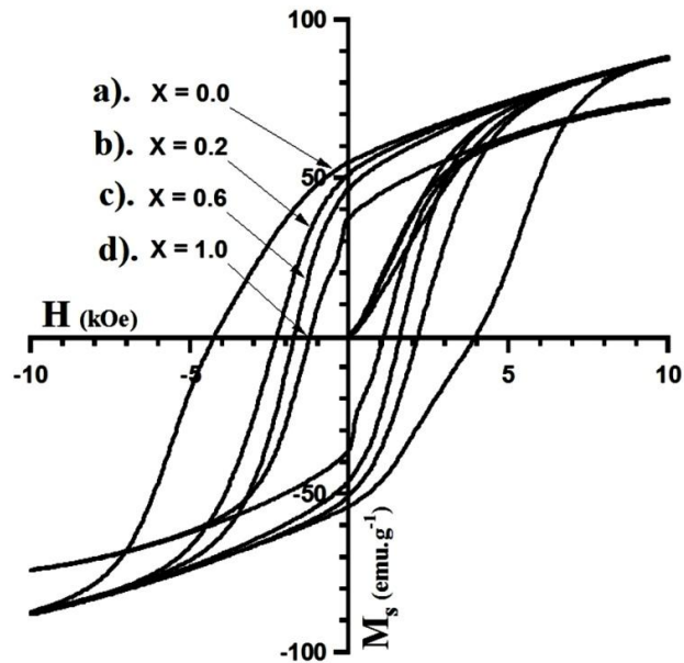
Figure 5. Room temperature hysteresis loop of (\text{Ba,Sr})_{0.5}\text{Fe}_{(12-2x)}(\text{ZnTi})_x\text{O}_{19} powder sample for (a) x = 0.0 , (b) x = 0.2 , (c) x = 0.6 , and (d) x = 1.0 .
