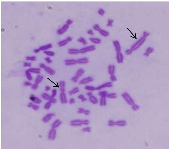
Fig. 3. A Giemsa-stained metaphasic cells containing two dicentrics (arrows) in lymphocytes of the whole blood irradiated with 2 Gy of gamma rays.
