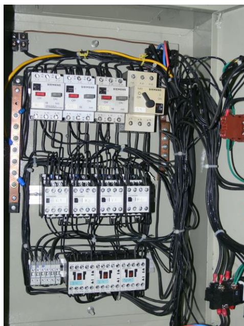
Gambar 7. Panel pengoperasian sistem injeksi bahan kimia
