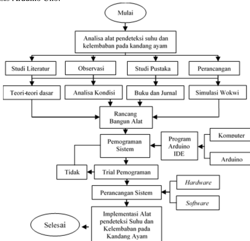
Gambar 1. Flowchart Penelitian
