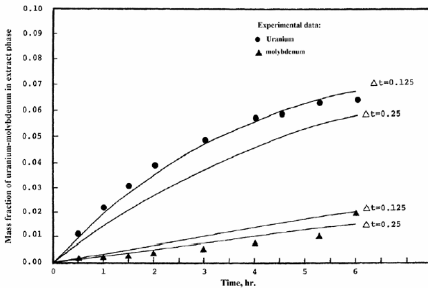
Fig. 5. Solvent Extraction
