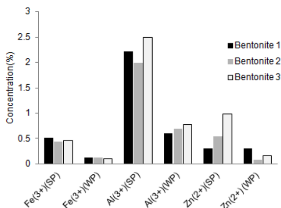
Fig 3. Release of Al 3+ , Fe 3+ and Zn 2+ from solids phase(SP) into the water phase (WP) in three types of bentonite
