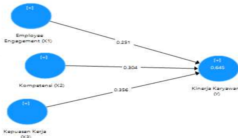
Gambar 2. Inner Model
