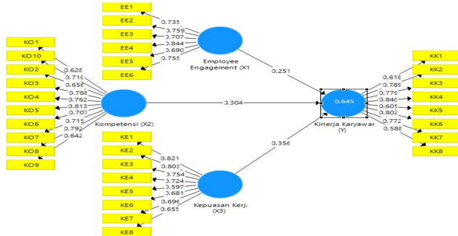
Gambar 1. Outer Model
