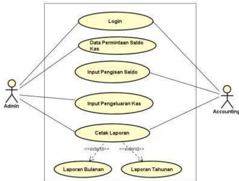
Gambar 2. Usecase Diagram
