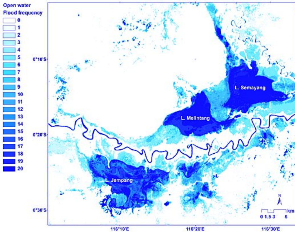
Figure 9. Inundation occurrence map of Mahakam cascade lakes from PALSAR images. The darkest colour indicates permanently inundated area.
