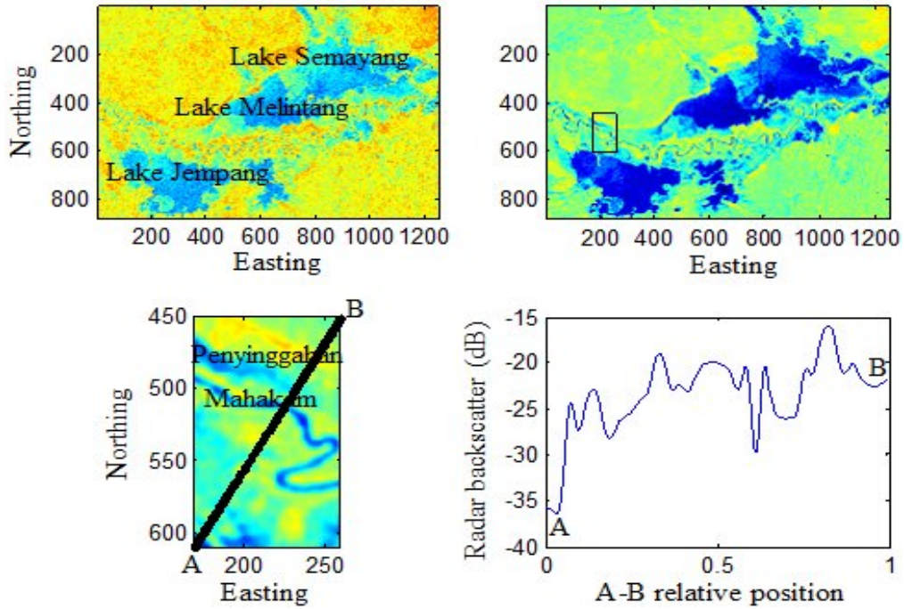
Figure 5. Two-dimensional image filtering of PALSAR image of the Mahakam lakes area. The top left is the original image, top right is the filtered image. Lower left image show a part of the image section from the shore of Lake Jempang across the river up to the northern floodplain in Penyinggahan and the corresponding radar backscatter shown in the lower right.
