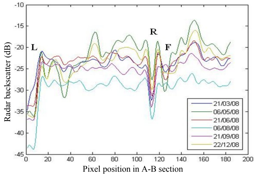
Figure 6. Backscatter value (dB) of filtered PALSAR images through floodplain (F) Mahakam river (R) and Lake Jempang (L) taken from the A-B sections in Fig. 5 in different image acquisition dates.
