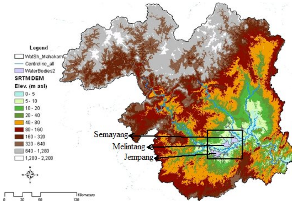
Figure 1. The Mahakam catchment upstream of the delta apex plotted on a digital elevation model obtained from SRTM data. The rectangle indicates the study area with the three main lakes.
