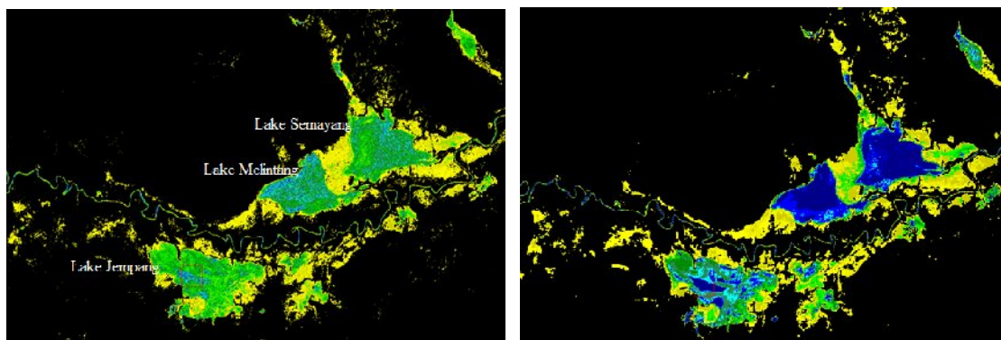
Figure 7. Colour map of flood frequency obtained from unfiltered 20 PALSAR images (left) and from filtered images using the enhanced Lee filter (right).
