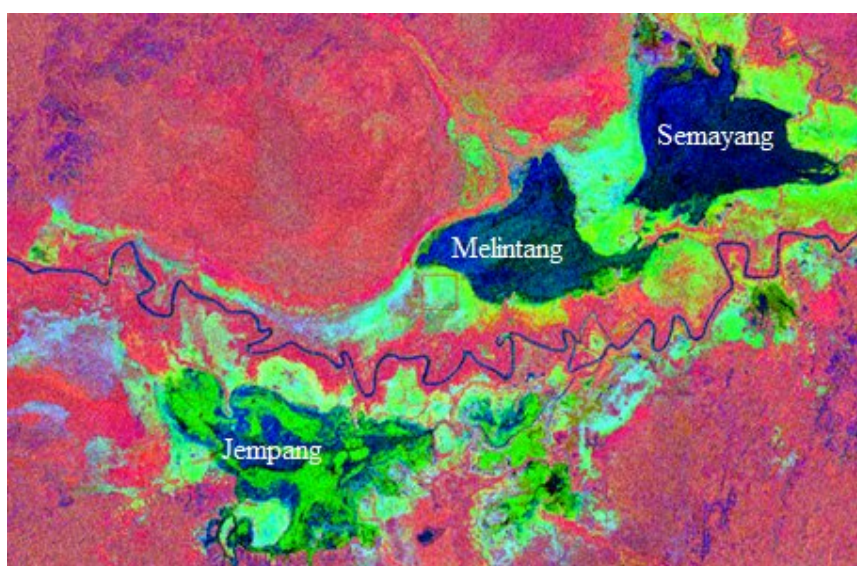
Figure 8. RGB colour composite of the first three PCA output of PALSAR images of the Mahakam lakes area. Bright green indicates floodplain inundation/lake extension. Dark blue indicates permanently inundated area.
