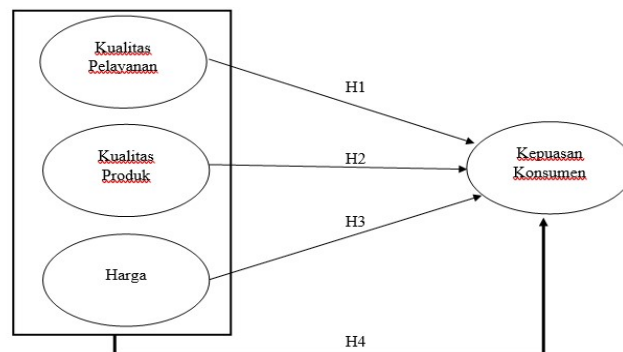
Gambar 3. Model Penelitian
