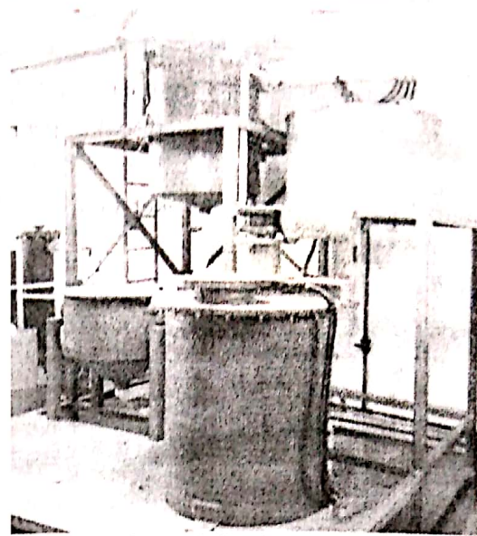
Gambar 3-2: Reaktor amoniasi
