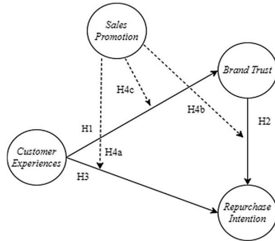
Gambar 1. Model Penelitian
