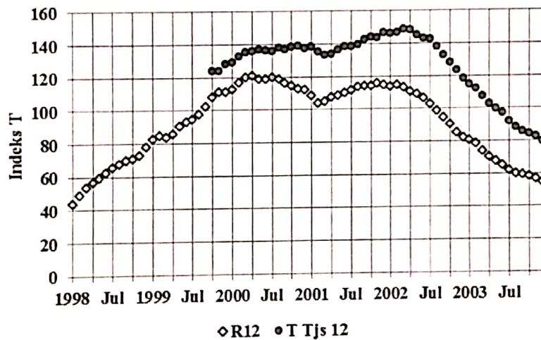
Gambar 2-1: Rata-rata berjalan ( moving average ) bilangan sunspot ( R_{12} ) dan Indeks T Tanjung Sari
