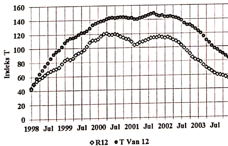
Gambar 2-2: Rata-rata berjalan ( moving average ) bilangan sunspot ( R_{12} ) dan Indeks T Vanimo
