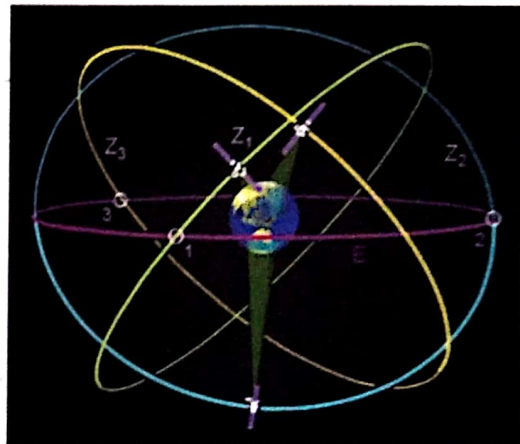
Gambar 2-2: Orbit QZSS (Sumber: Geometry of Zenith Satellites, 2001)
