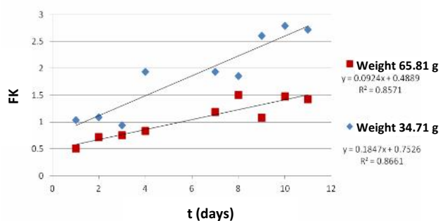
Figure 1. The gradient relationships between the uptake of 137 Cs and exposure time
