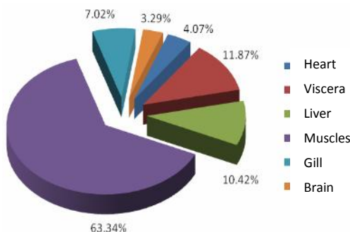
Figure 5. The distribution of 137 Cs accumulation inside the body of Cromileptes altivelis .
