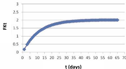
Figure 4. The estimation of CF ss of 137 Cs in Cromileptes altivelis with average body mass of 34.7 g
