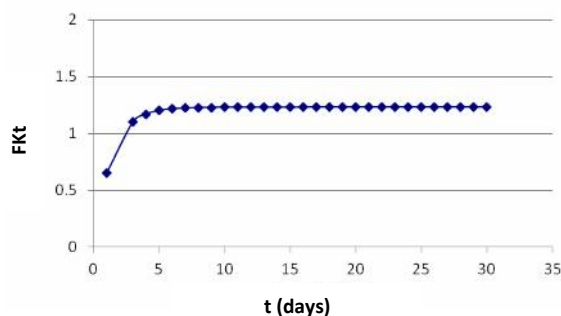
Figure 3. The estimation of CF ss of 137 Cs in Cromileptes altivelis with average body mass of 65.8 g
