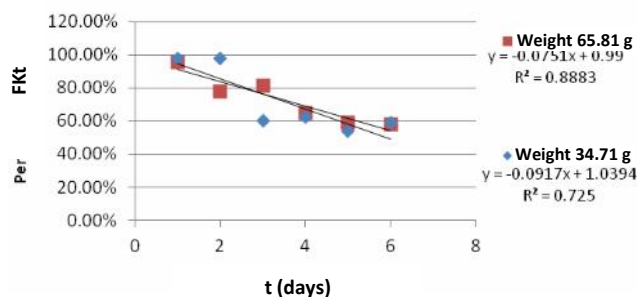
Figure 2. The gradient relationships between the rate of 137 Cs release and exposure time
