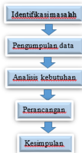
Gambar 1. Metode penelitian
