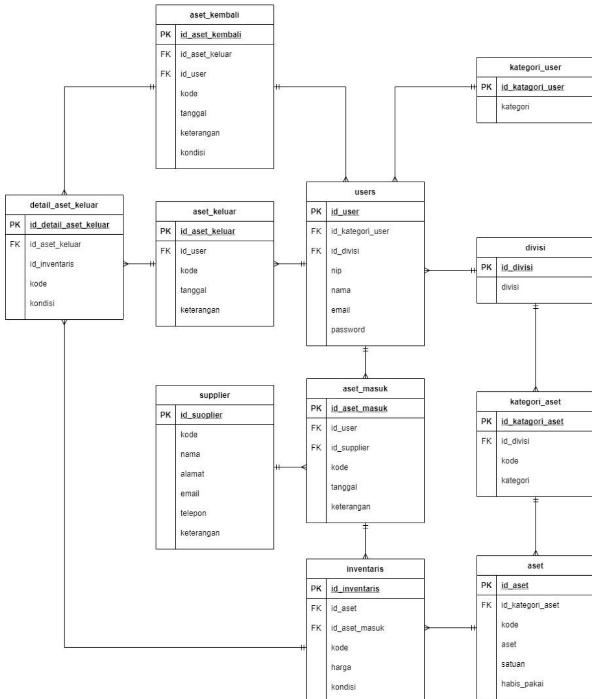
Gambar 5. Konseptual database
