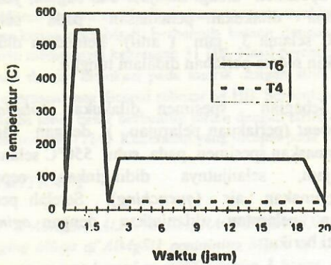
Gambar 2.b. Proses Aging
