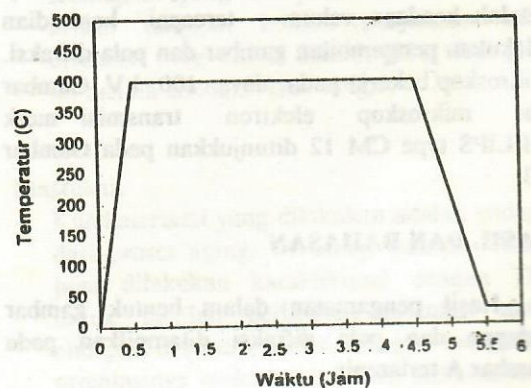
Gambar 2.a. Proses Anil
