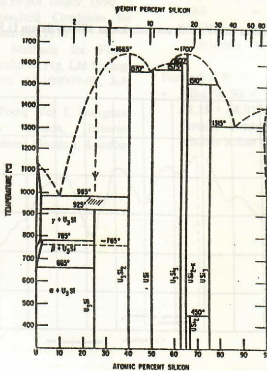
Gambar 4. Diagram fasa bahan bakar uranium silisida ( U_xSi_2 )
