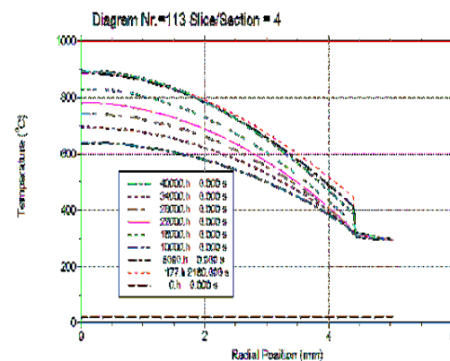
Fig. 5. Radial distribution of pin temperature at different irradiation time.
