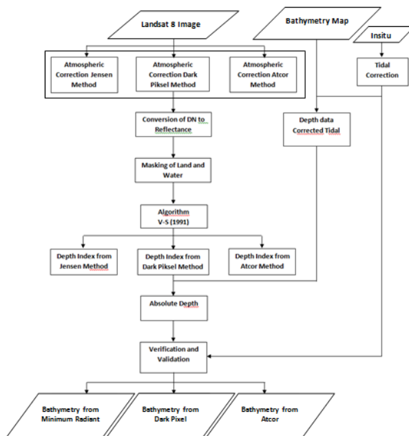
Figure 2-2: Research flowchart
